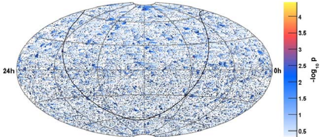
Figure 2.1-1. IceCube Detector Performance. Using declination and right ascension as coordinates, the map shows the probability for a point source of high-energy neutrinos with energies not readily accommodated by the steeply falling atmospheric-neutrino flux. Their energies range from 100 GeV to several 100 TeV. This map was obtained by operating IceCube with 40 strings for half a year. The “hottest spot” in the map has an excess of 7 events, an excursion from the atmospheric background with a probability of 10^{-4.4} . After taking into account trial factors, the probability to get a spot this hot somewhere in the sky is not significant. The map contains 6,796 neutrino candidates in the Northern Hemisphere and 10,981 down-going muons rejected to the 10^{-5} level in the Southern Hemisphere, shown as black dots.
